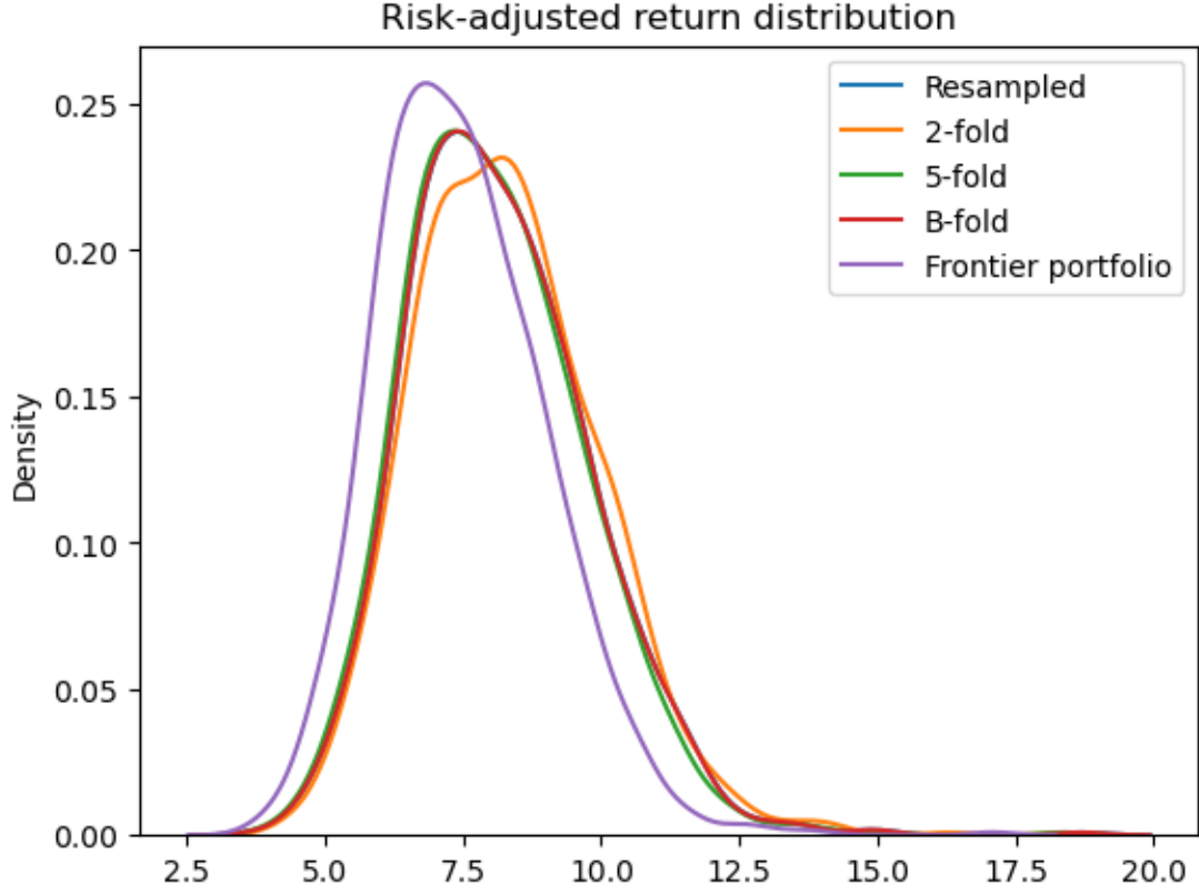
Figure 4: Distribution of the risk-adjusted returns.
