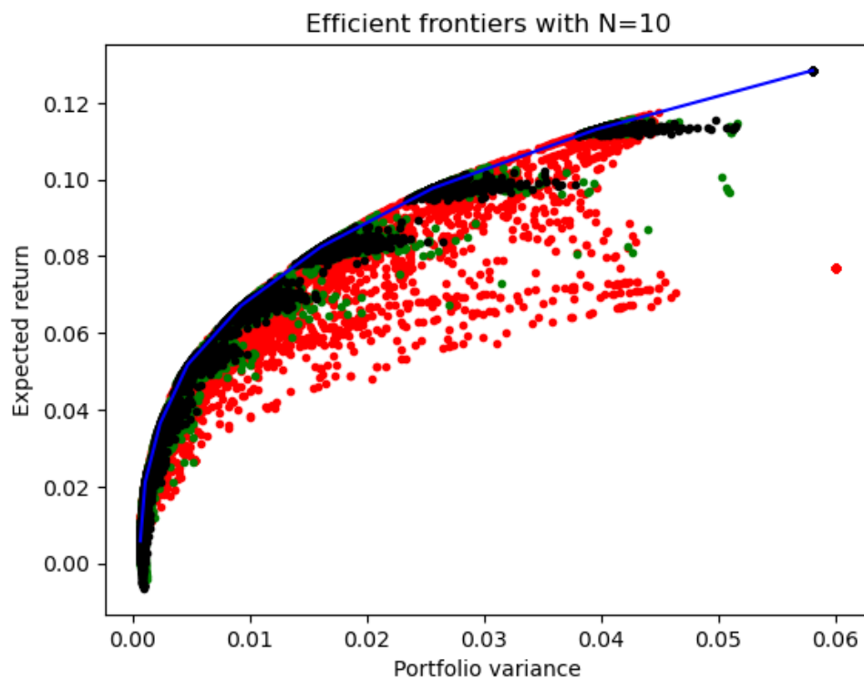
Figure 1: Efficient frontiers with N = 10 estimation observations.
