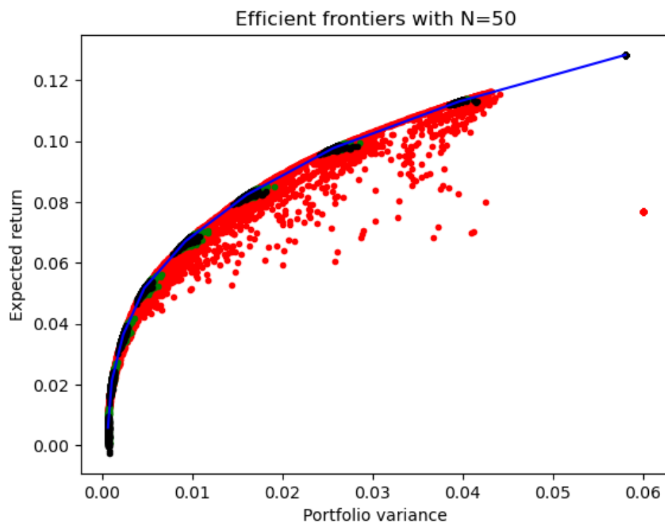
Figure 2: Efficient frontiers with N = 50 estimation observations.
