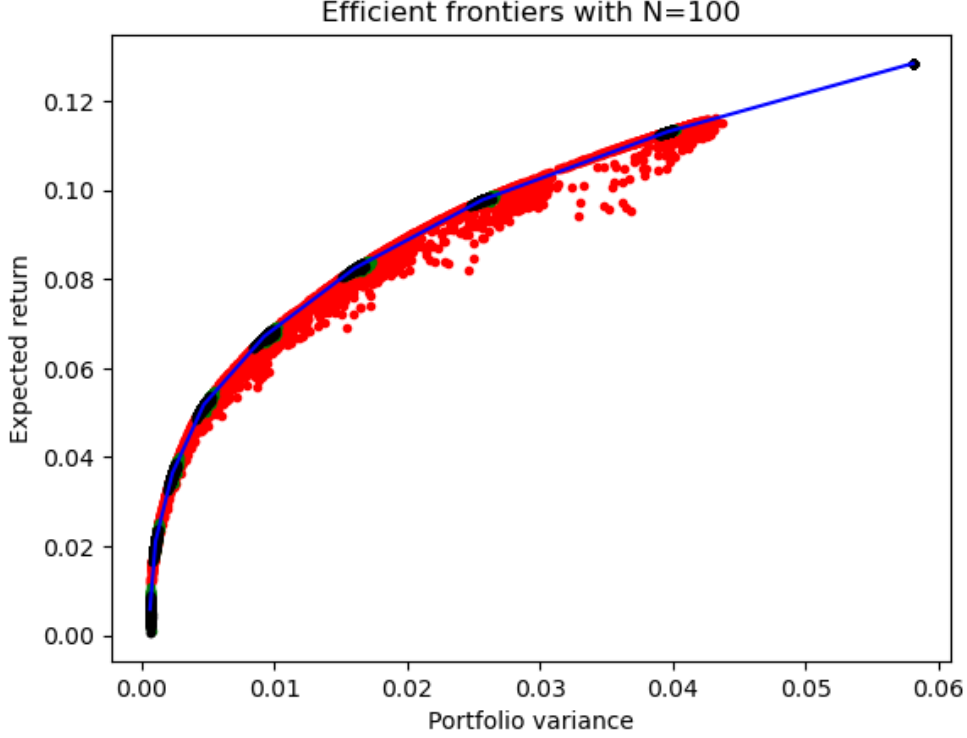
Figure 3: Efficient frontiers with N = 100 estimation observations.
