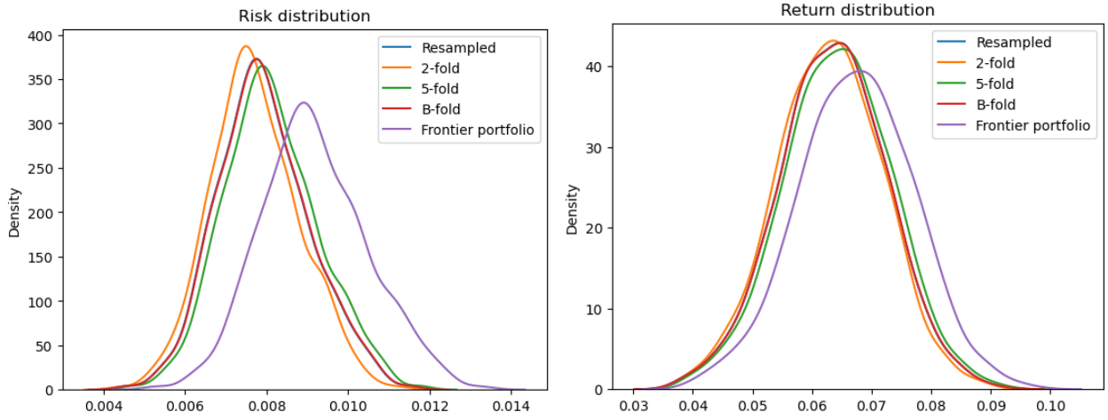
Figure 5: Out-of-sample risk and return distributions.
